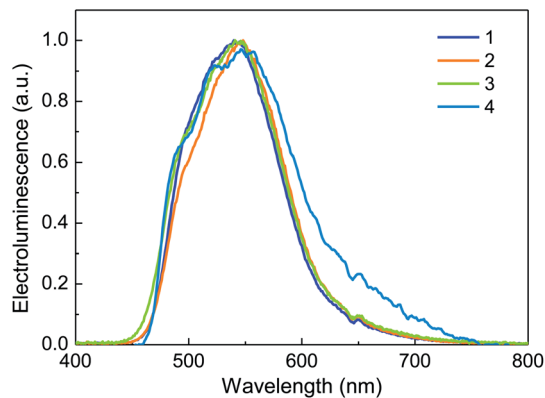
Fig. 8 Electroluminescence spectra obtained for LEC devices prepared with molecules 1–4 at 298 K.
