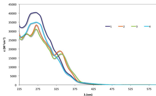
Fig. 2 UV-Vis absorption spectra of 1–4 recorded at 298 K in acetonitrile.
