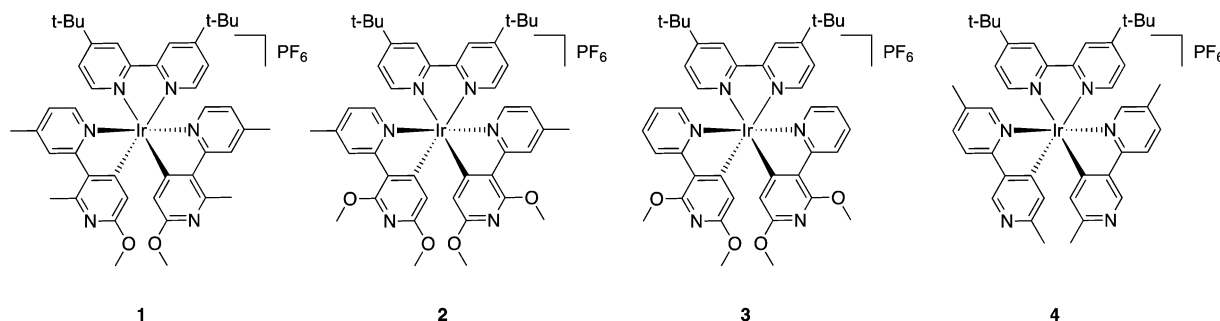
Chart 1 Structures of complexes 1–4 investigated in this study.
