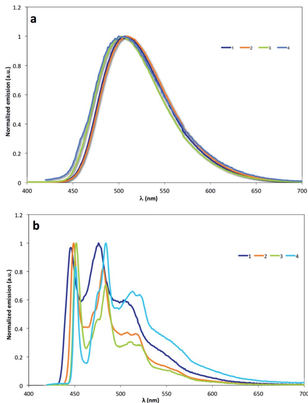
Fig. 3 Deaerated emission spectra for 1–4 recorded at (a) 298 K in acetonitrile and (b) 77 K in 2-MeTHF.
