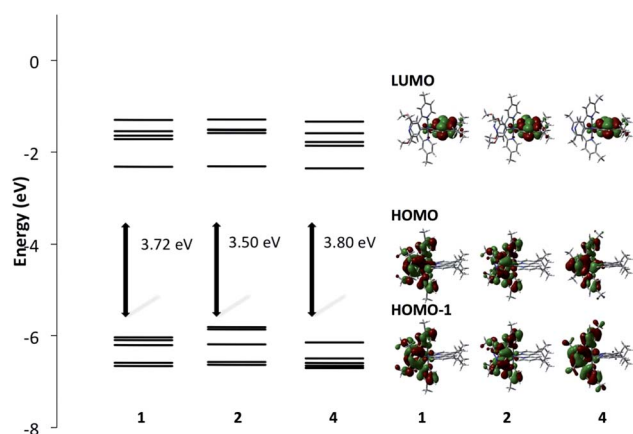
Fig. 5 Calculated energy level scheme for the Kohn–Sham orbitals between HOMO-4 and LUMO+4 of 1 , 2 and 4 and images electron density distribution for HOMO-1, HOMO and LUMO (isocontour value of 0.02 au).
