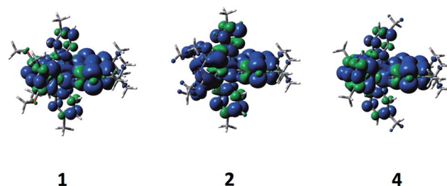
Fig. 6 Calculated spin density contours of the T 1 state for 1 , 2 and 4 (isocontour value of 0.0004 au).
