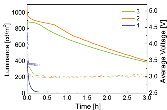
Fig. 7 Luminance (solid lines) and average voltage (dashed lines) for ITO/PEDOT : PSS/iTMC : IL (4 : 1)/Al devices driven at a pulsed current with an average current density of 100\text{ A m}^{-2} using a block wave at a frequency of 1000 Hz and a duty cycle of 50%.
