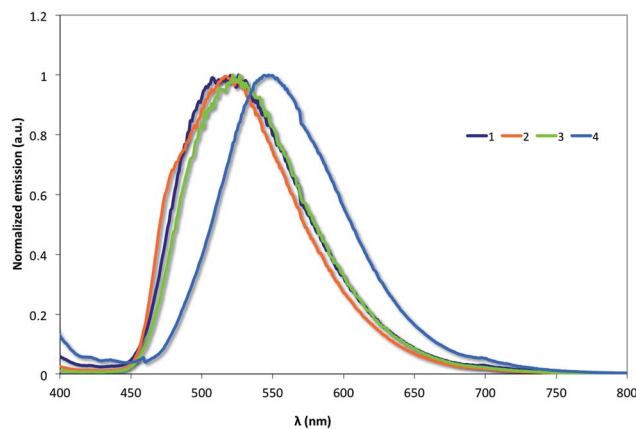
Fig. 4 Thin film emission spectra for 1–4 recorded at 298 K.
