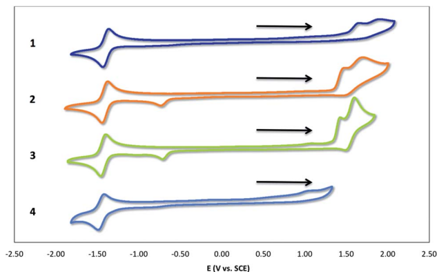
Fig. 1 Cyclic voltammetry for 1–4, recorded in deaerated acetonitrile; supporting electrolyte TBAPF 6 0.1 M. Working electrode: glassy carbon; counter electrode: Pt wire; reference electrode: Ag wire pseudo-reference. The Fc + /Fc couple was used as an internal standard and the potential was then referred to SCE ( E_{\text{SCE}} = E_{\text{Fc}^+/\text{Fc}} + 0.38 \text{ V} ). 16 — 1; — 2; — 3; — 4.
