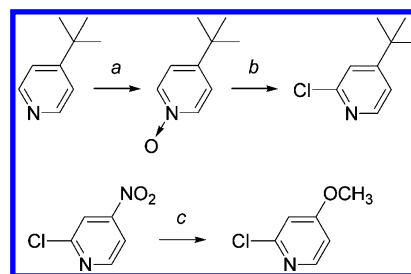
Scheme 3. Synthesis of 2-Chloropyridines a
